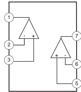
A BOARD IC401/IC531 LM393TD
